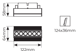
PRODUCT DRAWING
