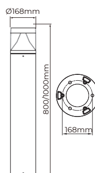
PRODUCT DRAWING
