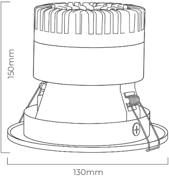
PRODUCT DRAWING
