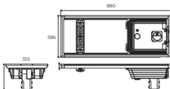
PRODUCT DRAWING
