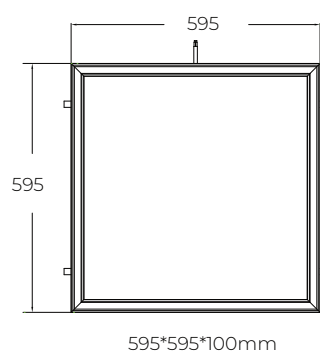
PRODUCT DRAWING
