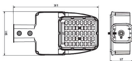
PRODUCT DRAWING
