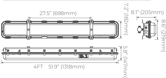
PRODUCT DRAWING
