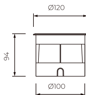
PRODUCT DRAWING
