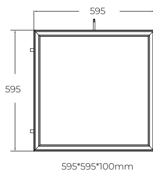
PRODUCT DRAWING
