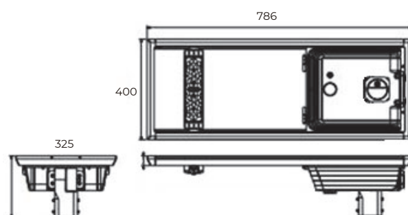
PRODUCT DRAWING
