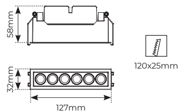
PRODUCT DRAWING
