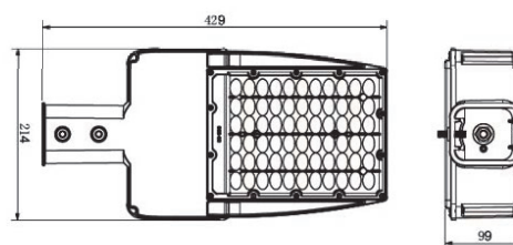
PRODUCT DRAWING
