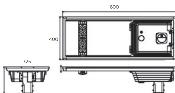
PRODUCT DRAWING
