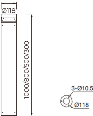
PRODUCT DRAWING
