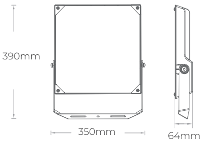
PRODUCT DRAWING
