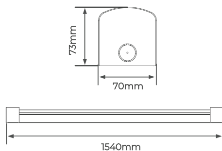
PRODUCT DRAWING
