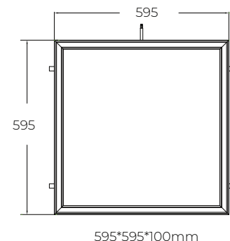
PRODUCT DRAWING
