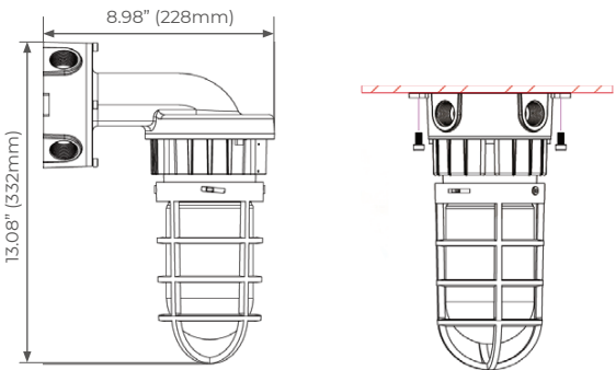
PRODUCT DRAWING
