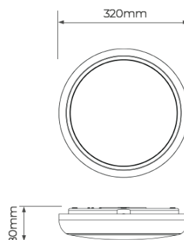
PRODUCT DRAWING
