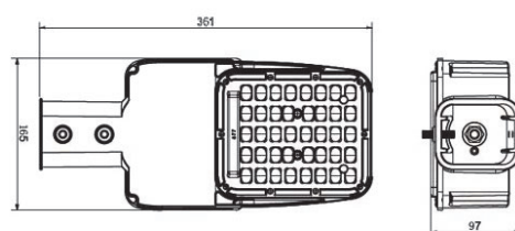
PRODUCT DRAWING
