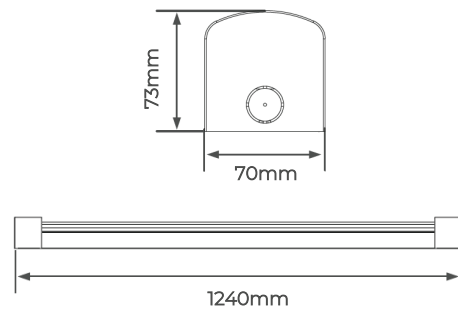
PRODUCT DRAWING
