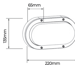
PRODUCT DRAWING
