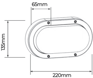
PRODUCT DRAWING
