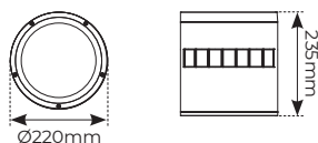
PRODUCT DRAWING
