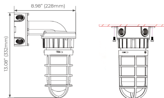
PRODUCT DRAWING
