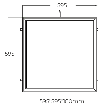
PRODUCT DRAWING
