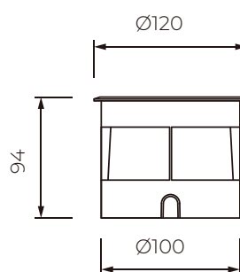
PRODUCT DRAWING
